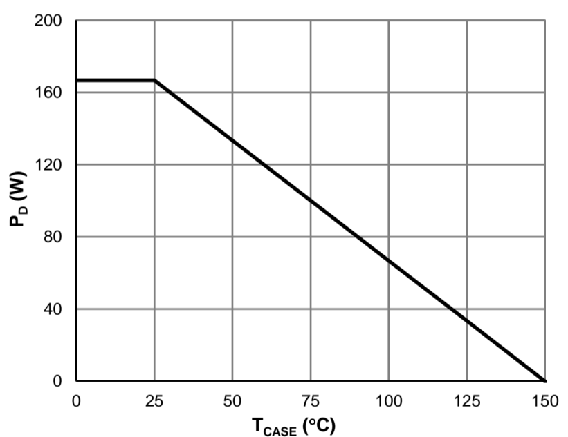
Figure 10: Power De-rating
