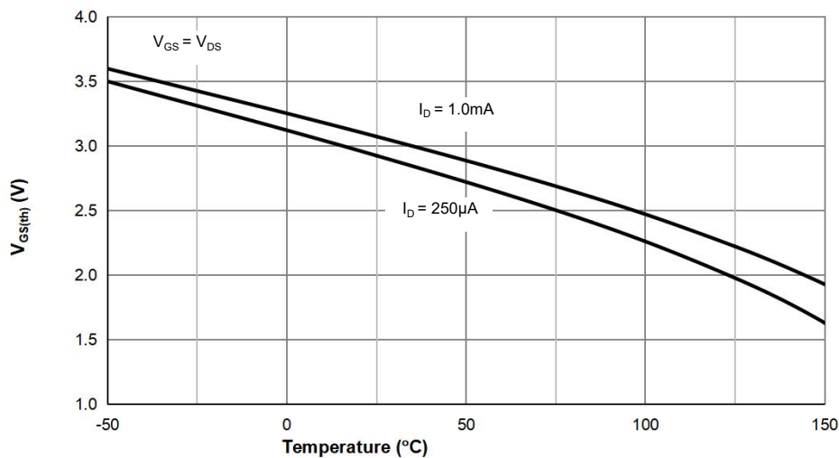
Figure 5: V_{GS(th)} vs. Junction Temperature
