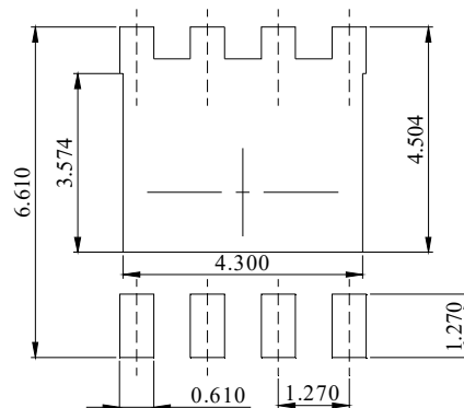
DIMENSIONS: MILLIMETERS
