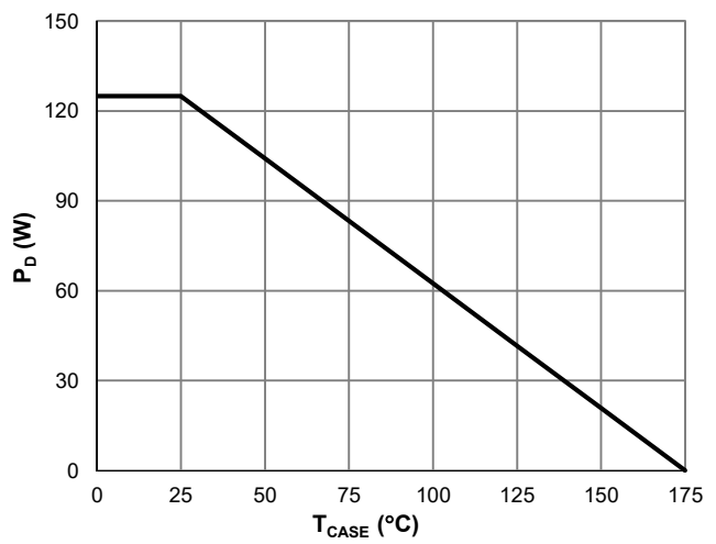
Figure 8: Power De-rating
