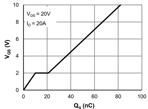
Gate Charge
