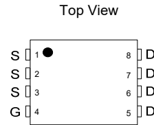
Pin Configuration
