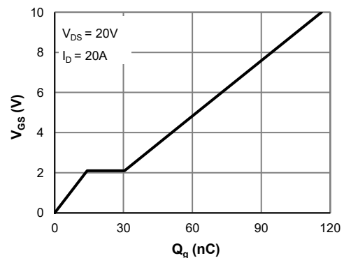
Gate Charge
