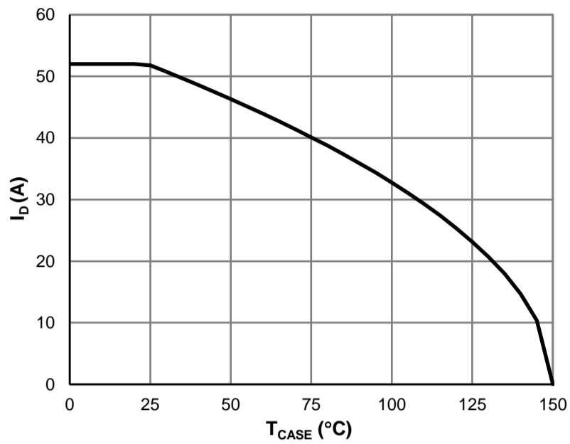
Figure 7: Current De-rating
