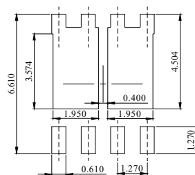
DIMENSIONS:MILLIMETERS
