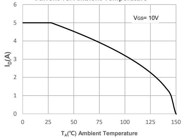
Figure 10: Maximum Continuous Driain Current vs. Ambient Temperature
