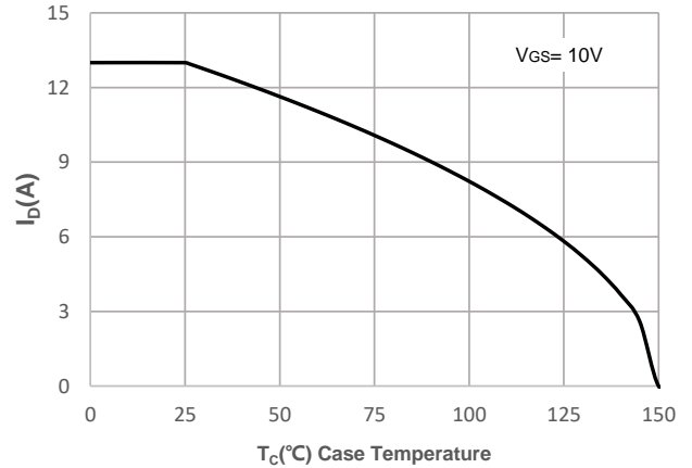
Figure 10: Maximum Continuous Drivan Current vs. Case Temperature
