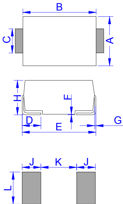
DO-214AA (SMB)
