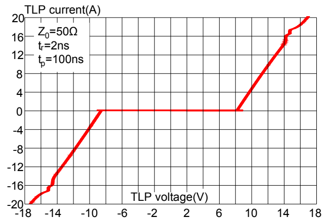
FIG.6: TLP Measurement
