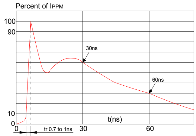
FIG.4: ESD clamping
