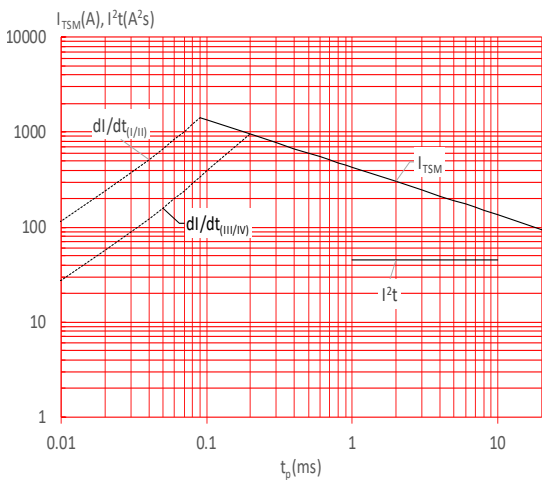
FIG.5: Non-repetitive surge peak on-state current for a sinusoidal pulse with width t_p < 20\text{ms} , and corresponding value of I^2t ( I - II: di/dt < 100\text{A}/\mu\text{s} ; III-IV: di/dt < 70\text{A}/\mu\text{s} )
