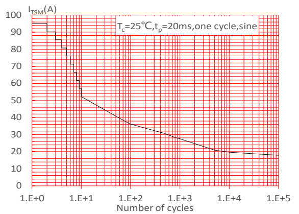
FIG.6: Non-repetitive surge peak on-state current for a sinusoidal pulse with width t_p < 20\text{ms} , and corresponding value of I^2t ( I - II : di/dt < 100\text{A}/\mu\text{s} ; III-IV : di/dt < 70\text{A}/\mu\text{s} )
