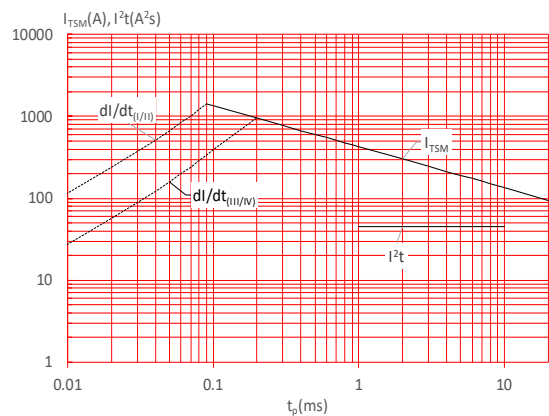
FIG.6: Non-repetitive surge peak on-state current for a sinusoidal pulse with width t_p < 20\text{ms} , and corresponding value of I^2t ( I - II : di/dt < 100\text{A}/\mu\text{s} ; III-IV : di/dt < 70\text{A}/\mu\text{s} )
