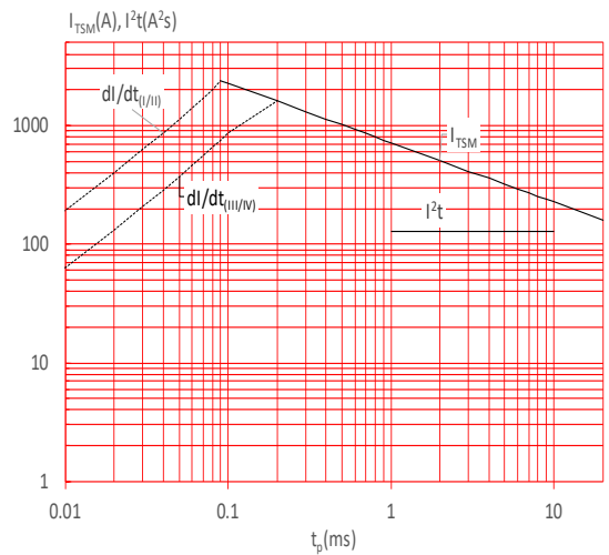
FIG.6: Non-repetitive surge peak on-state current for a sinusoidal pulse with width t_p < 20\text{ms} , and corresponding value of I^2t (I - II: dl/dt < 100\text{A}/\mu\text{s} ; III-IV: dl/dt < 50\text{A}/\mu\text{s} )
