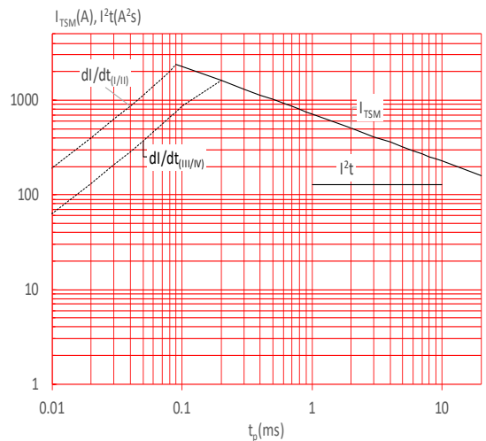
FIG.6: Non-repetitive surge peak on-state current for a sinusoidal pulse with width t_p < 20\text{ms} , and corresponding value of I^2t (I - II: di/dt < 100\text{A}/\mu\text{s} ; III-IV: di/dt < 50\text{A}/\mu\text{s} )
