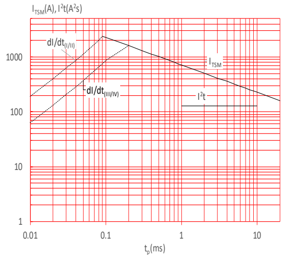
FIG.6: Non-repetitive surge peak on-state current for a sinusoidal pulse with width t_p < 20\text{ms} , and corresponding value of I^2t (I - II: di/dt < 80\text{A}/\mu\text{s} ; III-IV: di/dt < 40\text{A}/\mu\text{s} )
