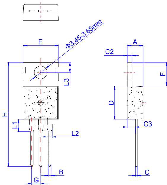
TO-220C
